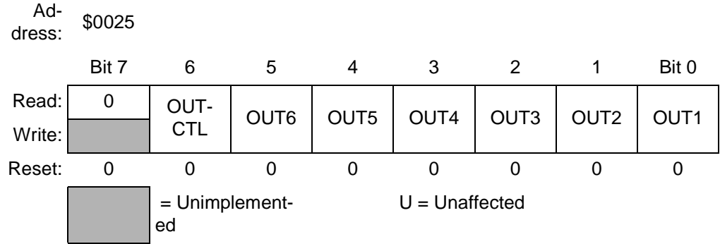
Figure 9-42. PWM Output Control Register (PWMOUT)
