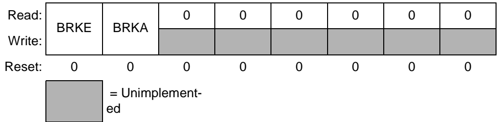
Figure 20-3. Break Status and Control Register (BRKSCR)
