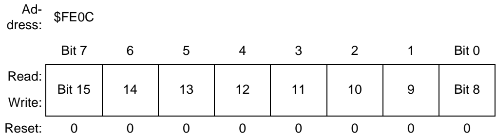
Figure 20-4. Break Address Register High (BRKH)
