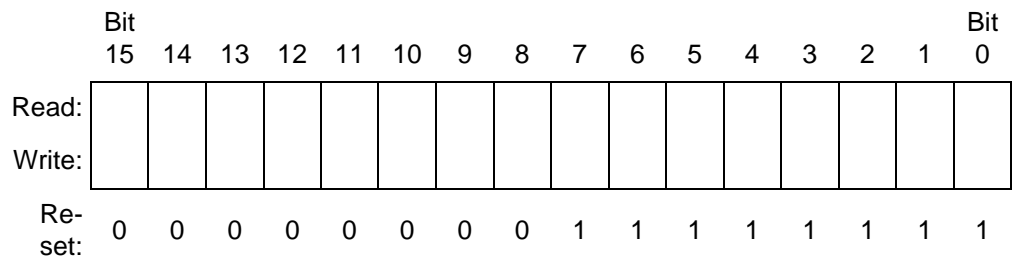
Figure 6-4. Stack Pointer (SP)
