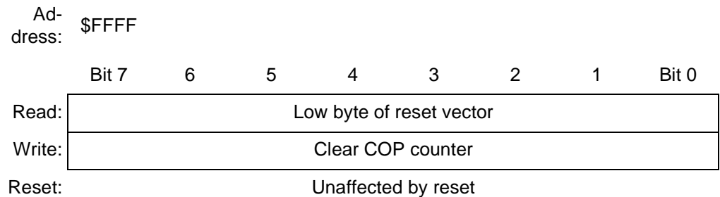
Figure 15-3. COP Control Register (COPCTL)
