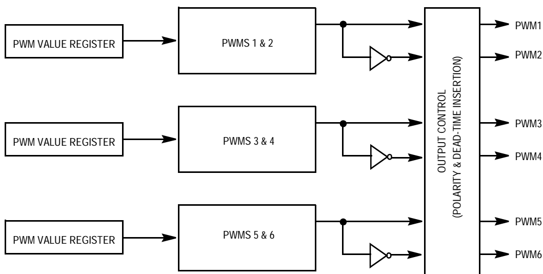
Figure 9-11. Complementary Pairing
