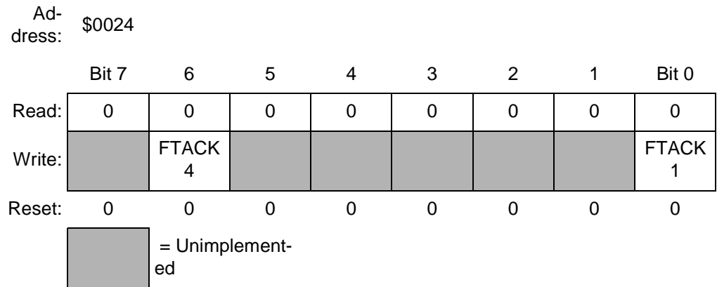
Figure 9-41. Fault Acknowledge Register (FTACK)
