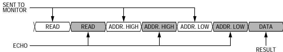
Figure 10-4. Read Transaction
